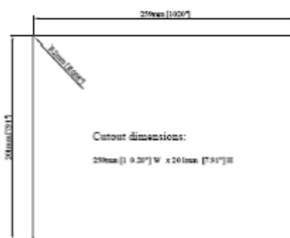
Panel Cutout
