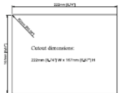
Panel Cutout
